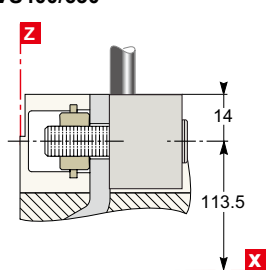
CVS400/630
